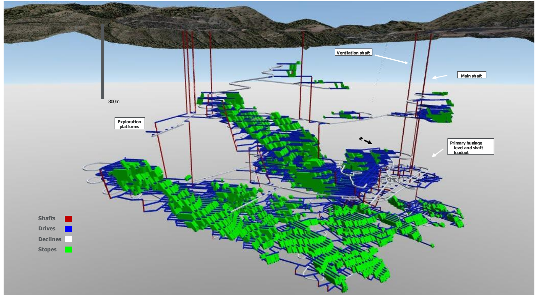
Taylor Deposit underground mine design
