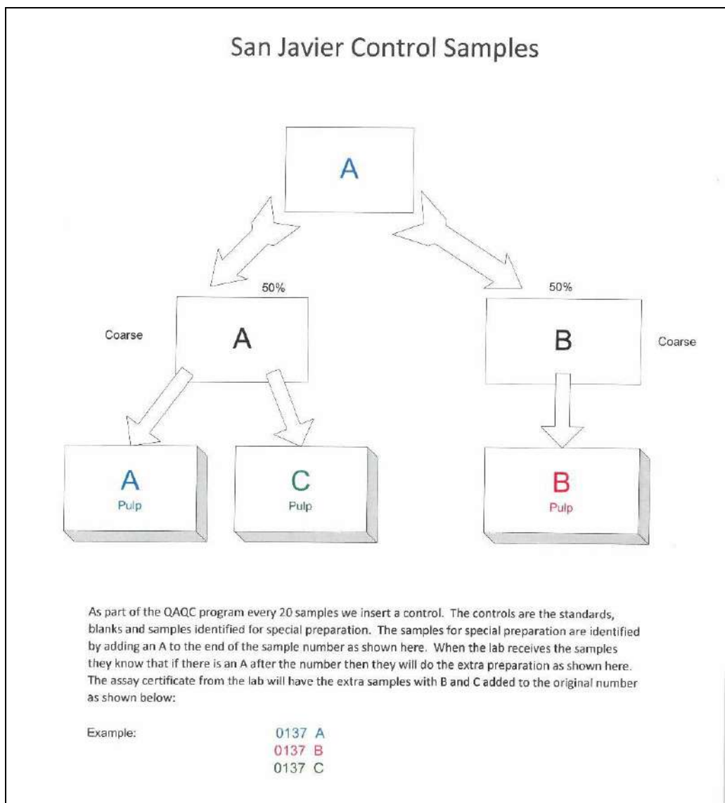
Figure 12-6: San Javier Control Samples
