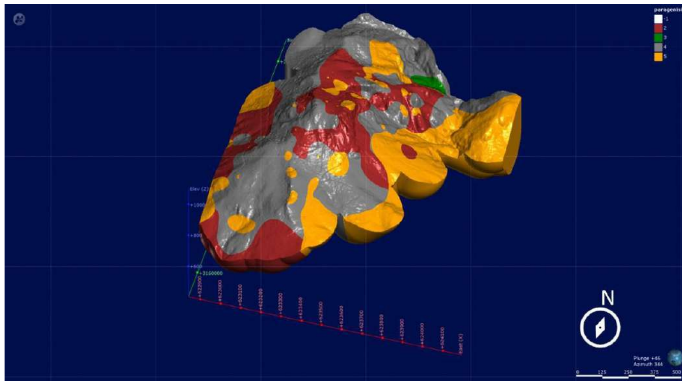
Figure 14-4: Surface Expression of Alteration Units (Barksdale, 2021)
