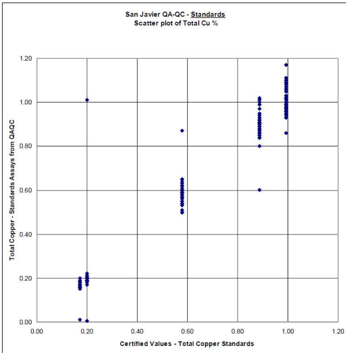
Figure 12-4: Total Copper Standards
