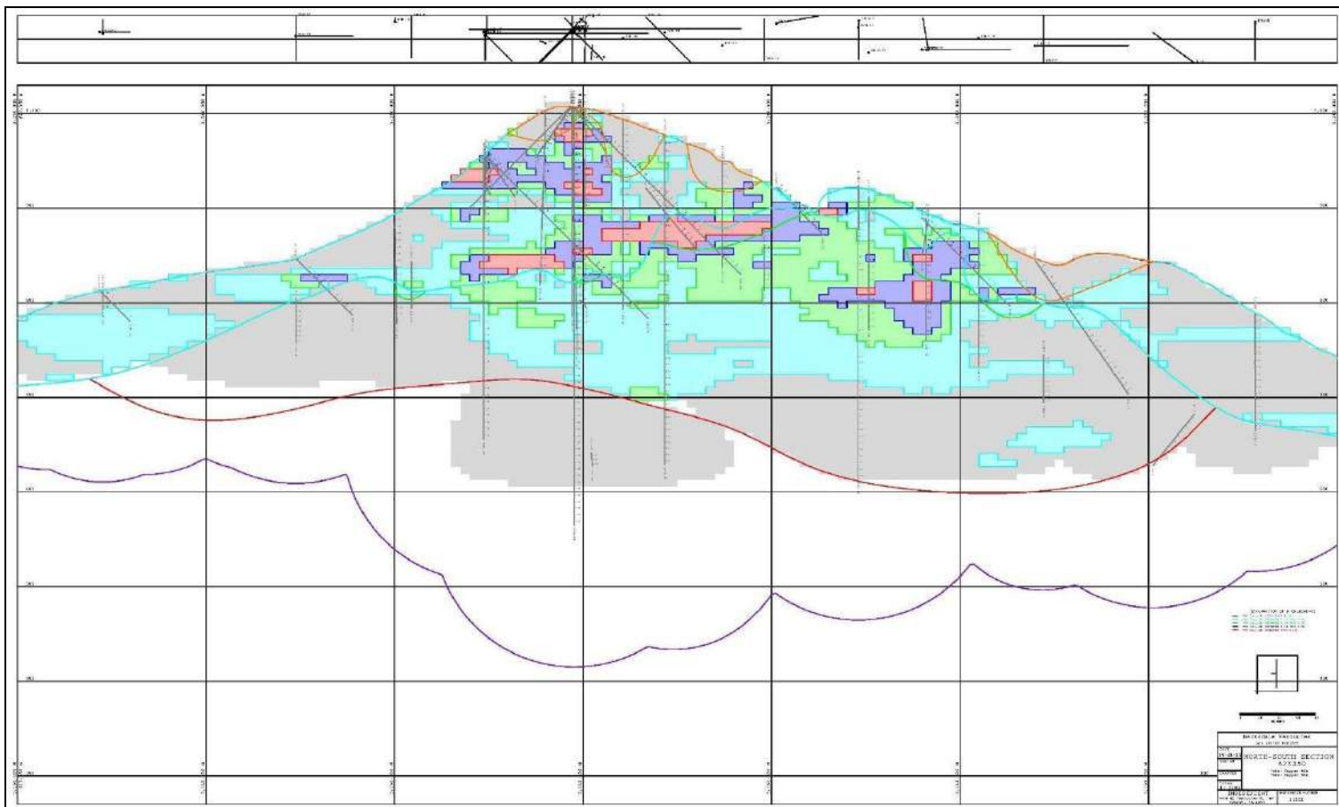
Figure 14-13: North-South Section 623,300E Showing TCu Grades
