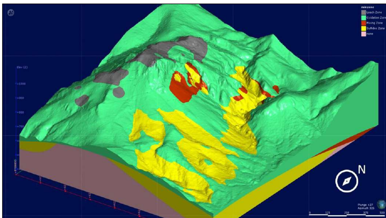
Figure 14-3: Mineralization Zones Surface Expression as a 3D View (Barksdale, 2021)
