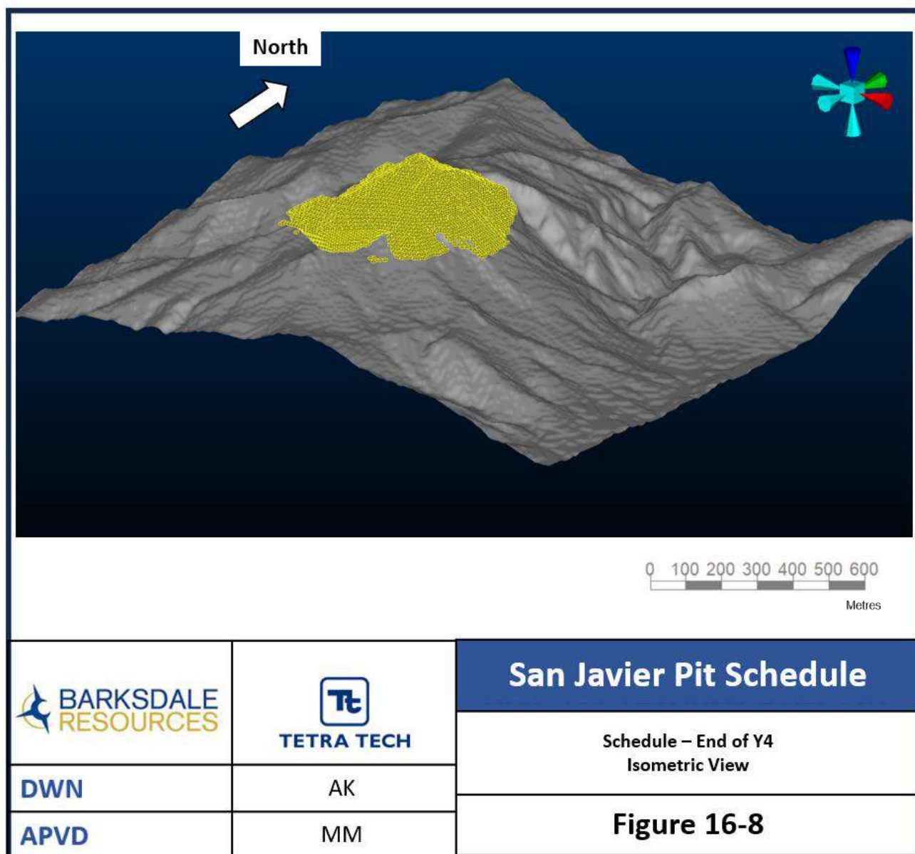
Figure 16-8: Pit Progression End of Year 4 (Isometric View Looking North-West)
