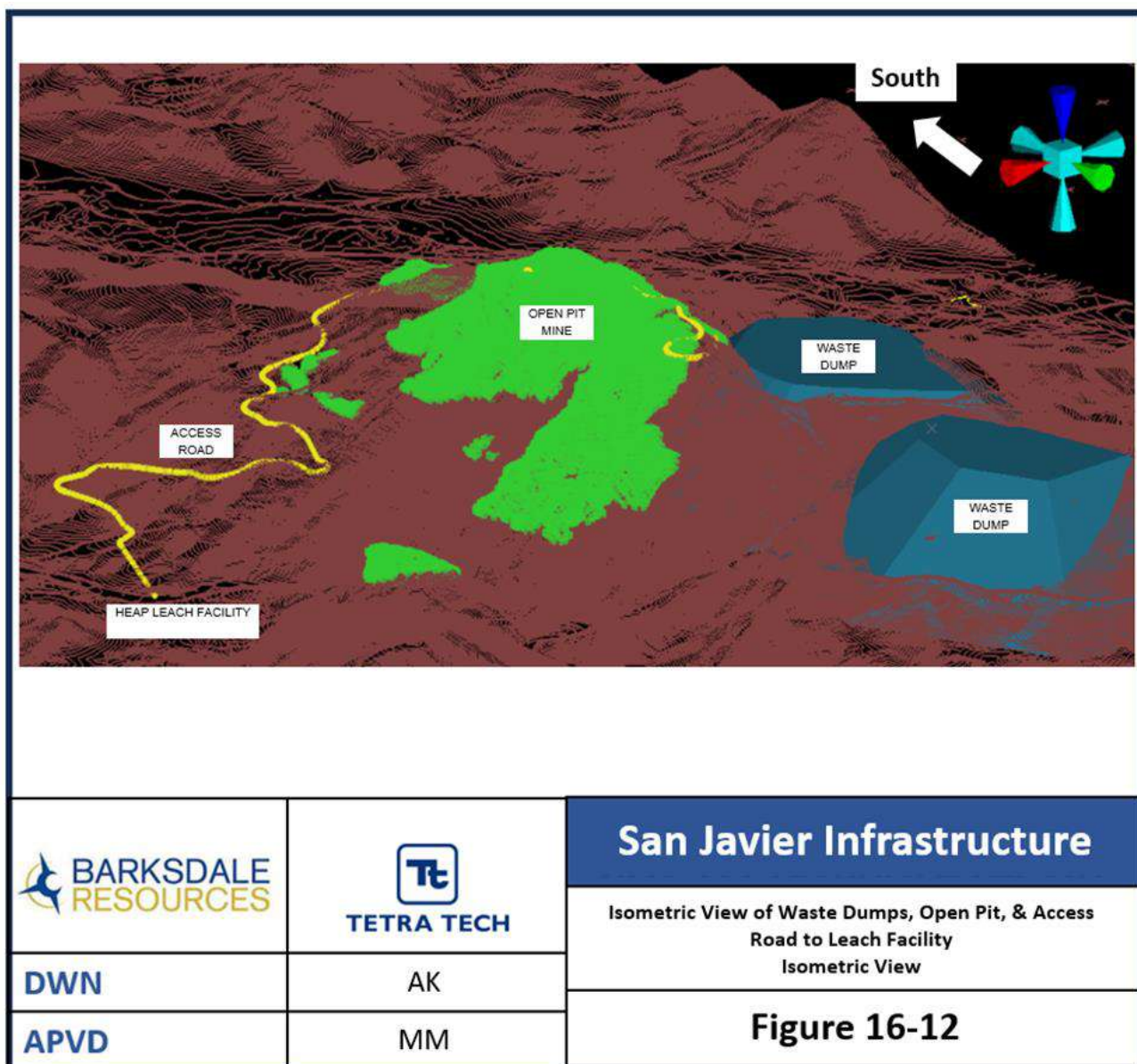
Figure 16-12: Isometric View of Waste Dumps, Open Pit Mine, and Access Road to Leach Facility
