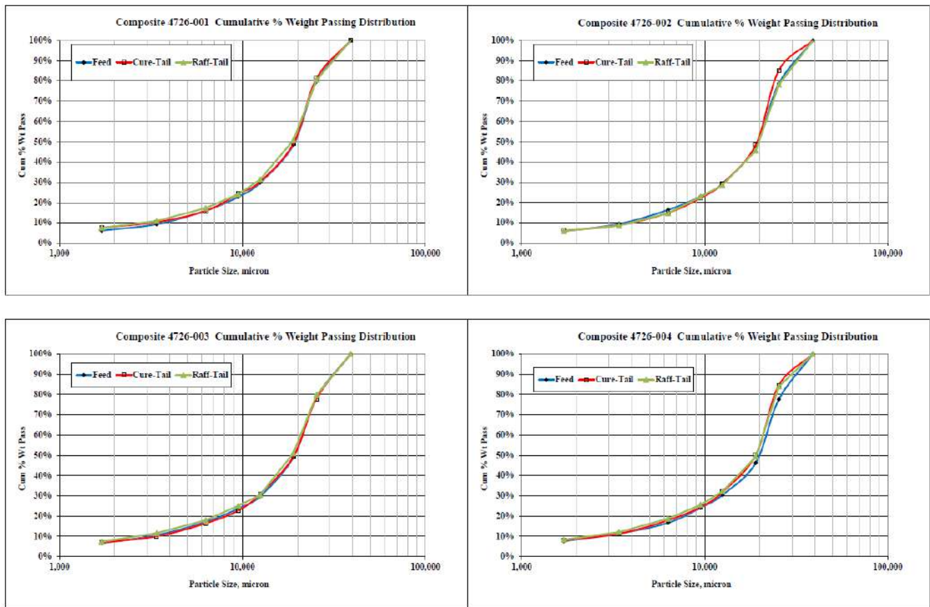
Figure 13-10: Particle Size Distribution for Feed and Tailings for Each Column Test (SND Consulting, 2022)
