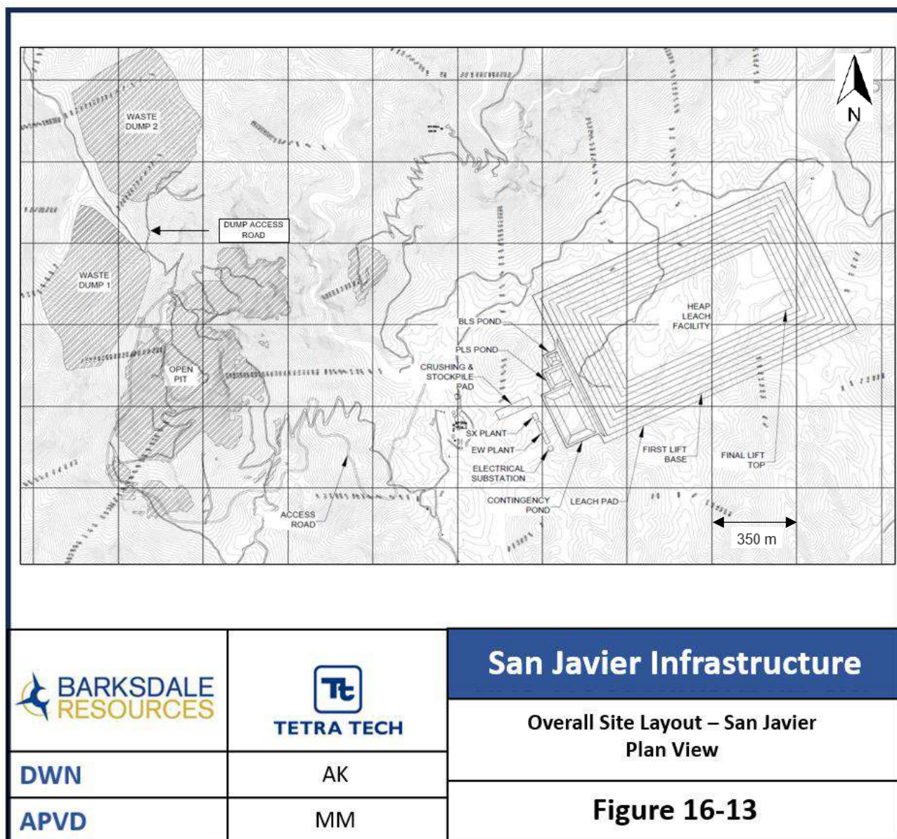
Figure 16-13: Overall Site Layout for the San Javier Project
